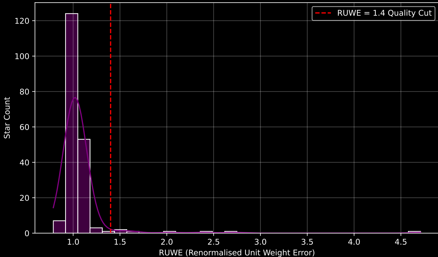
GAPOGEE DR17 Field [020+14] RUWE Distribution (n= 195)
