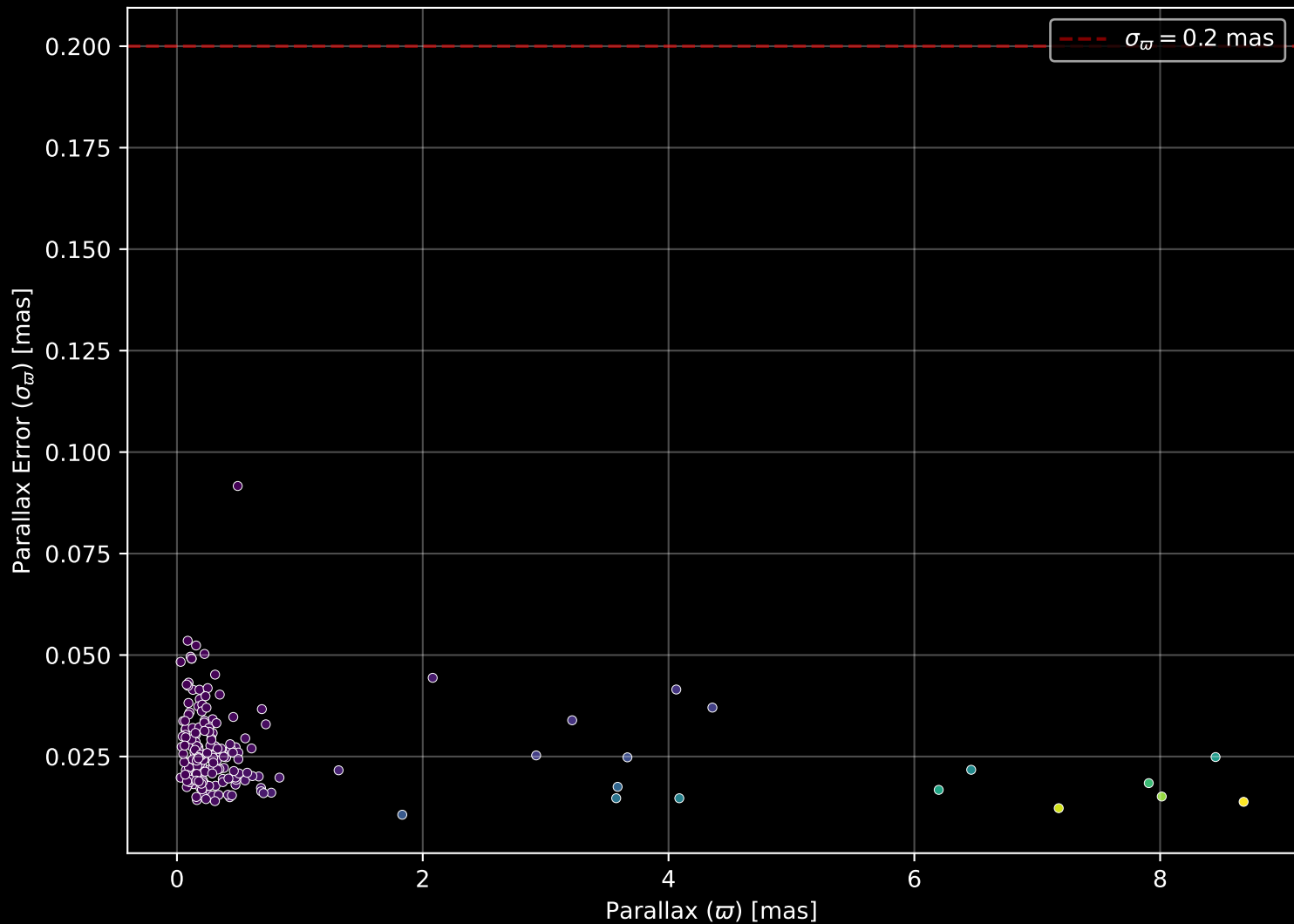
APOGEE DR17 Field: [020+14] Parallax Quality (n= 195)
