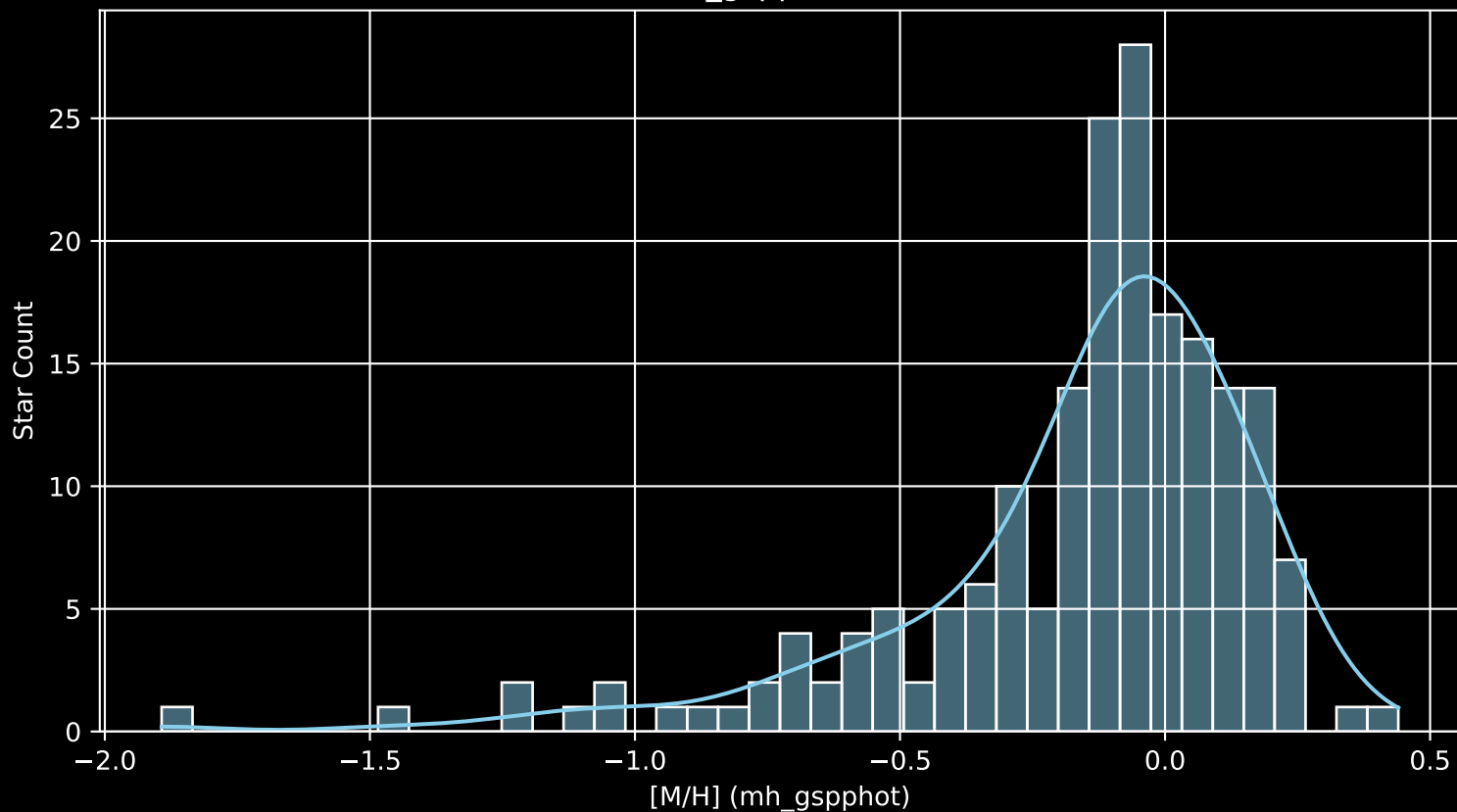
APOGEE DR17 Field: [020+14 [M/H] (mh_gspphot) (n= 192)
