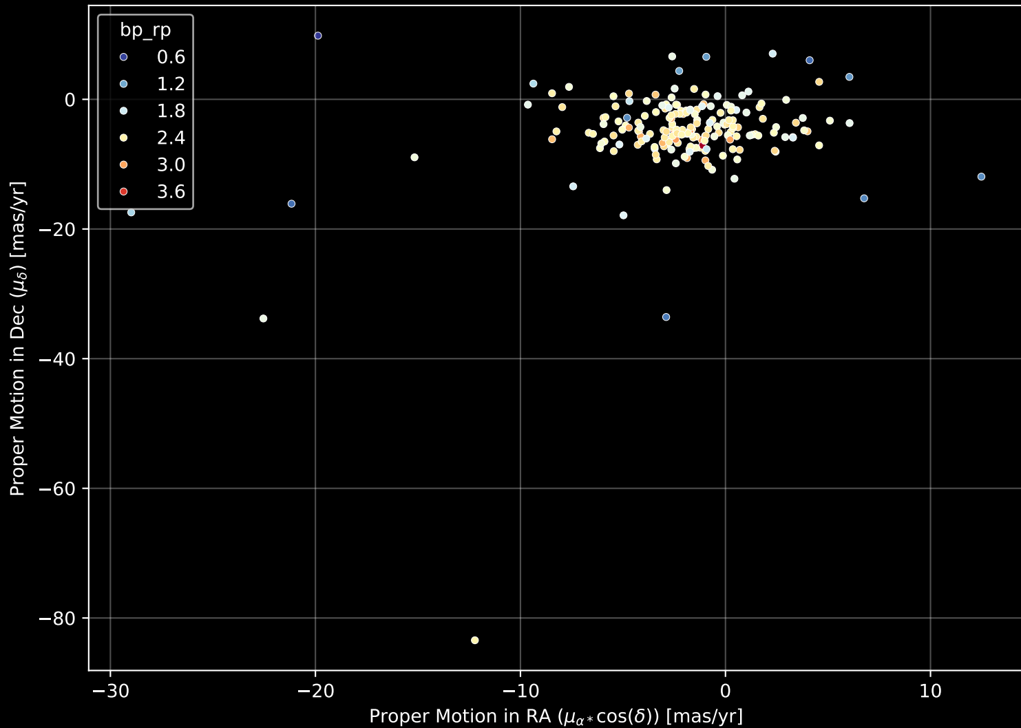
APOGEE DR17 Field: [020+14] Proper Motion Diagram (n= 195)
