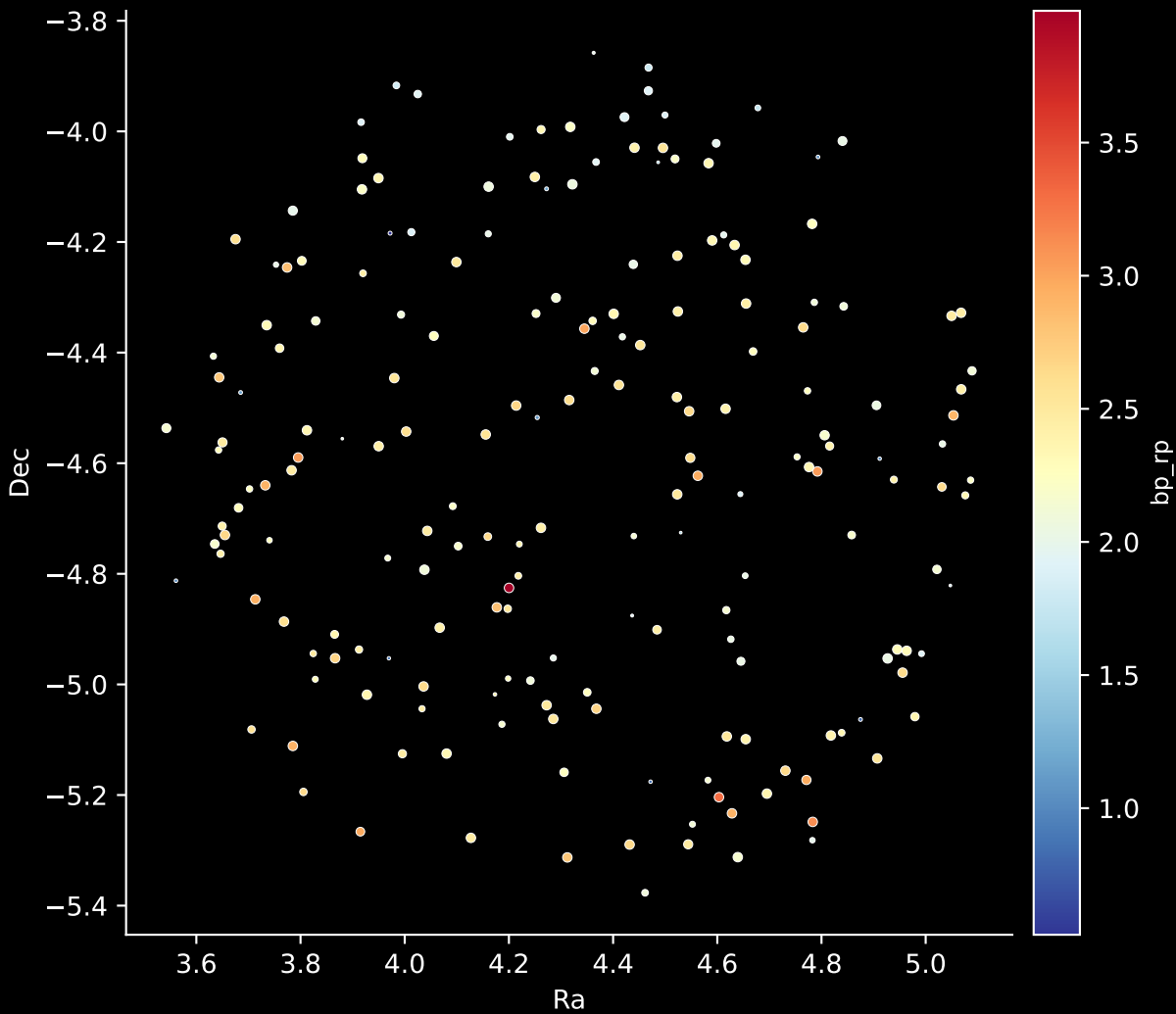
APOGEE DR17 Field: [020+14] Stars: 195
