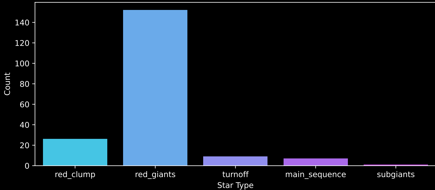
APOGEE DR17 Field: [020+14] Count plot of Star Type
